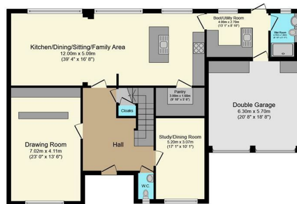
Ground Floor Floor area 122.5 sq.m. (1,319 sq.ft.)
